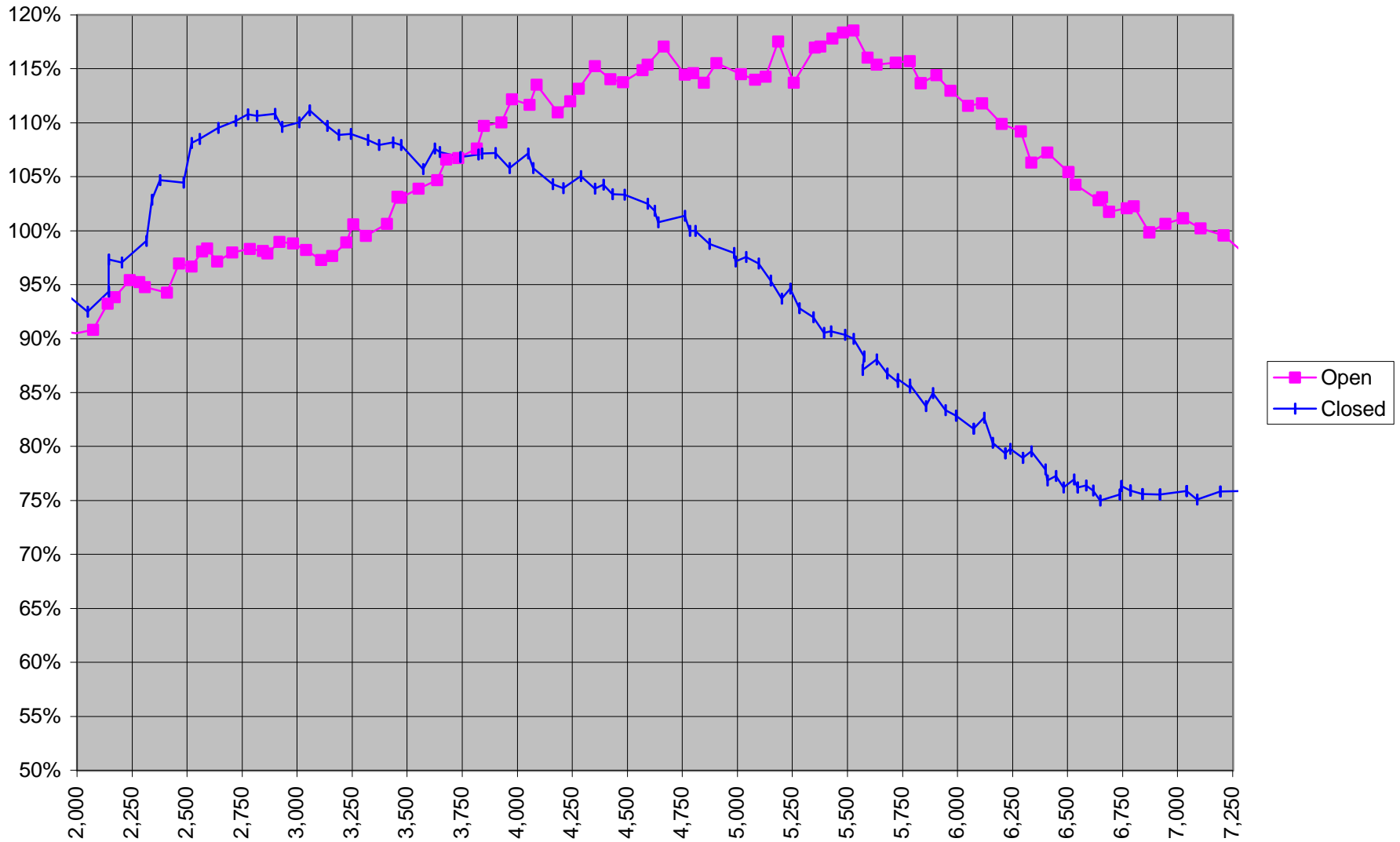
Load (VE - or torque production potential) vs. RPM for a Stock SHO
